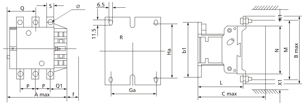
LC1-D115~620 LC1-ND115~150
