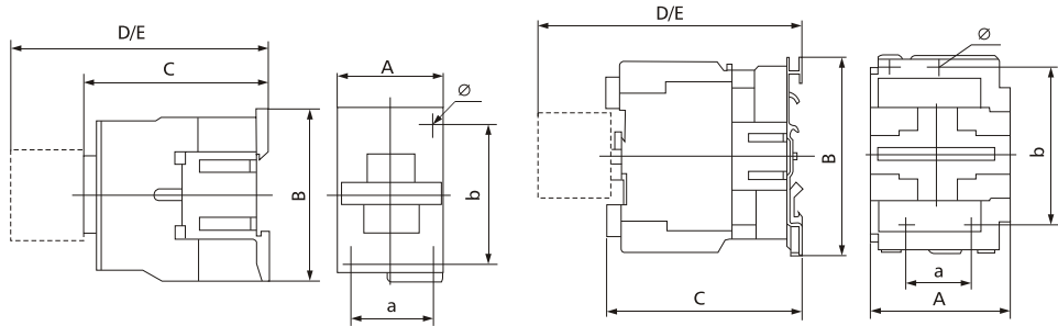
LC1-D09~32 LC1-ND09~32
